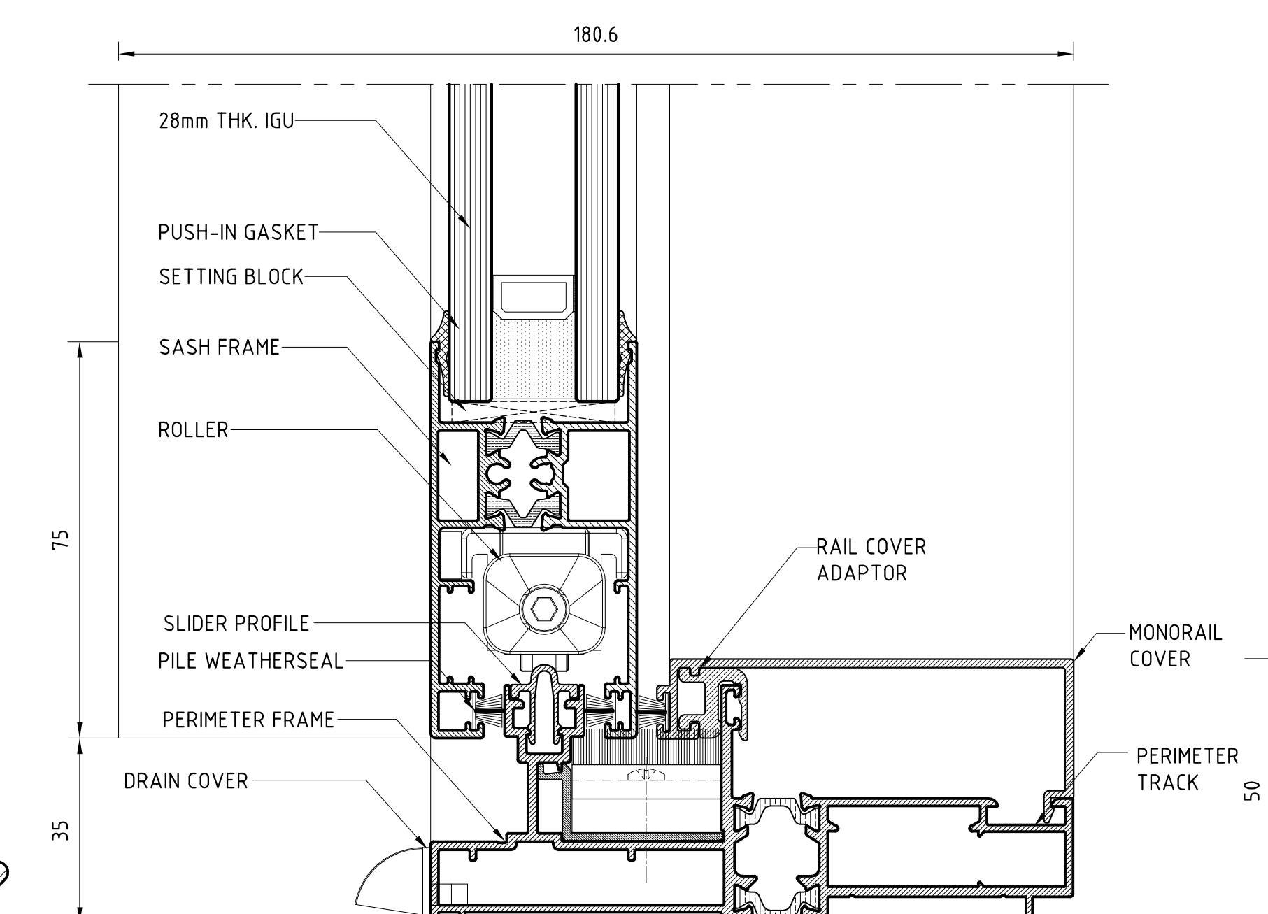
BOTTOM RAIL DETAIL
